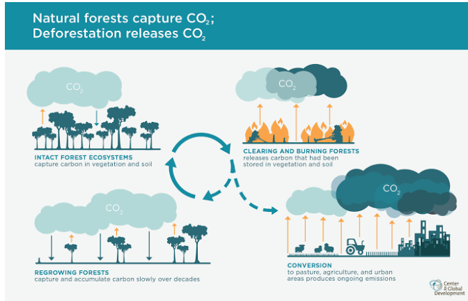
Fig. 2. The processes that release carbon dioxide into the atmosphere and its interaction with the environment.
