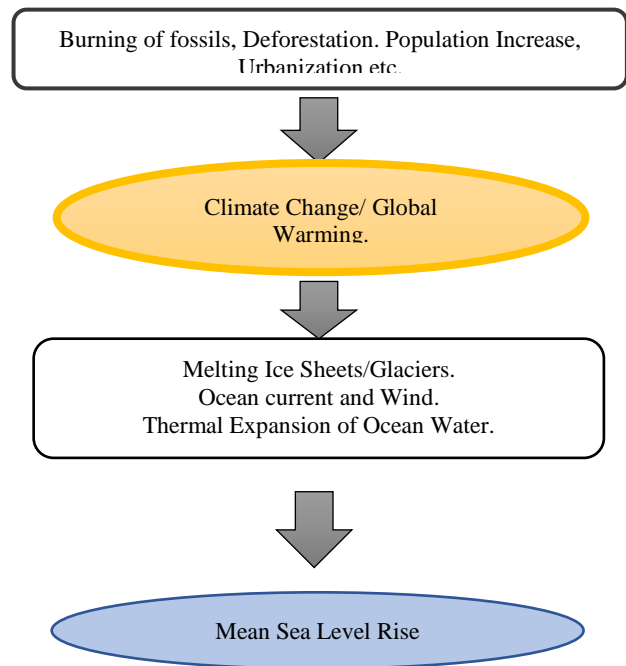
Fig. 1. Some of the factors inducing Mean Sea Level Rise
